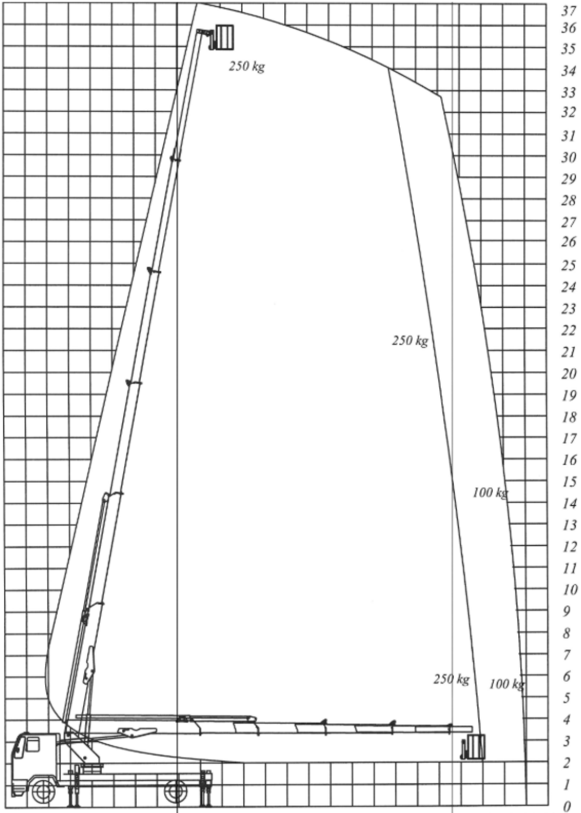
HT 37 TELESCOPIC PLATFORM WORKING DIAGRAM
